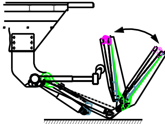
Folding process
