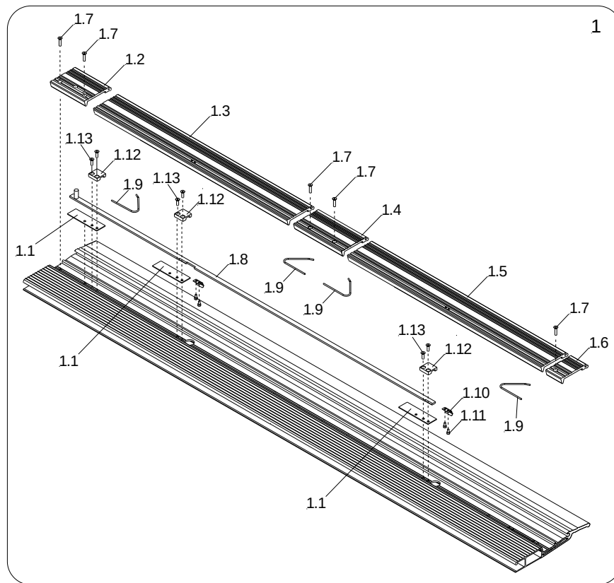
7.1 – CART STOPS ALUMINUM PLATFORMS
