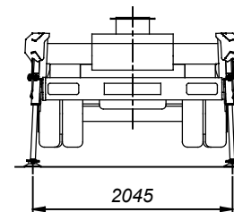
WORK AREA 01 P200TXE-E-PLUS ON IVECO DAILY 35S14 WB 4100
